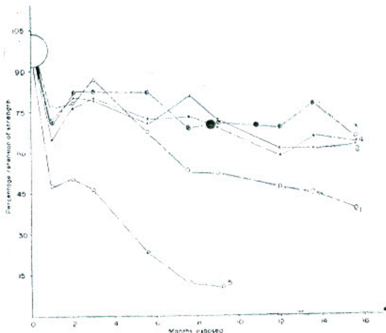
Fig. 8: Weather of treated cotton twines on exposure to sunlight. Place: Cochin. 1. Cutch + Carboleneum 2. Cutch + Testalin + Carboleneum 3. Cutch fixed with K_2Cr_2O_7 + Carboleneum 4. Cutch fixed with CuSO_4NH_3 + Carboleneum 5. 15% Arigal C + 0.25% Arigal PMP
