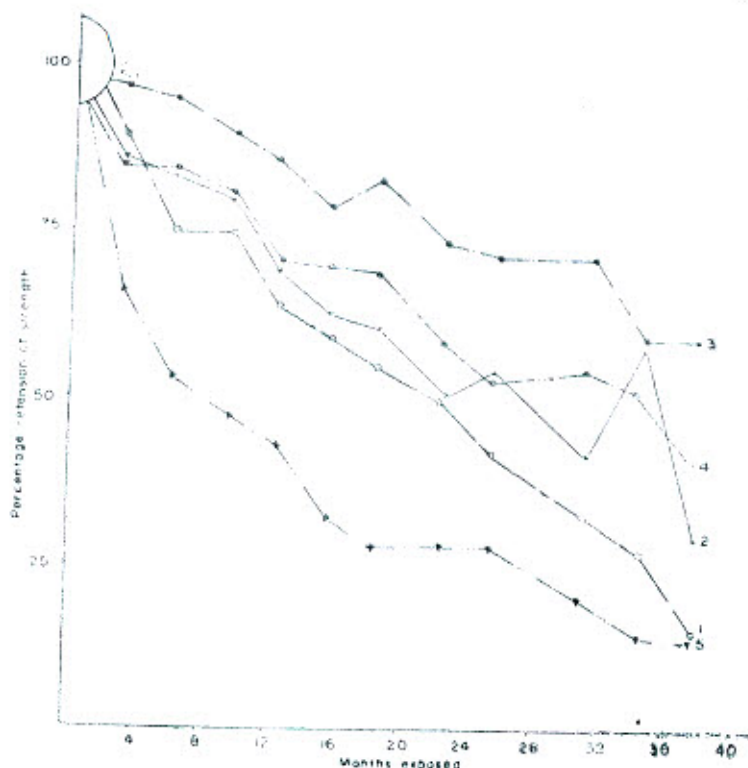
Fig. 7: Weathering of treated cotton twines on exposure to sunlight. Place: Hamburg 1. Cutch + Carboleneum 2. Cutch + Testalin + Carboleneum 3. Cutch fixed with K_2Cr_2O_7 + Carboleneum 4. Cutch fixed with CuSO_4.NH_3 + Carboleneum 5. 15% Arigal C + 0.25% Arigal PMP.
