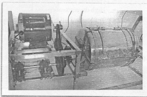
Fig.7 Fish de-scaling machine with fixed drum speed
