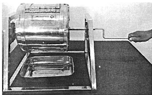
Fig.8. Fish de-scaling machine hand operated
