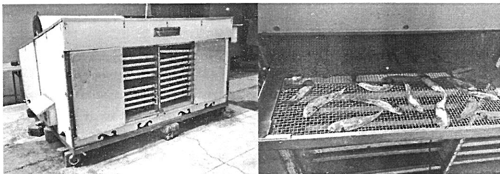
Fig.5. CIFT Solar-Cabinet Dryer with Electrical back-up
