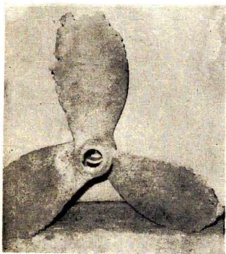
Fig. I Dezincification and erosion attack on marine propeller.
