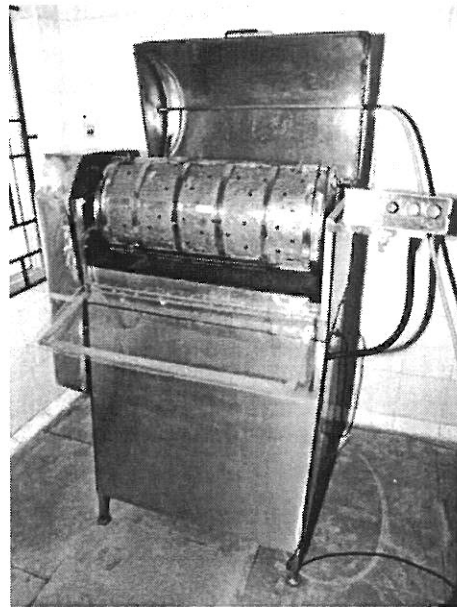
Fig.6 Fish de-scaling machine with variable drum speed
