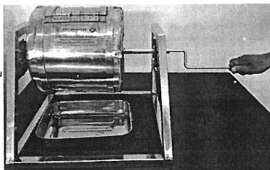
Fig.7 Fish de-scaling machine hand operated
