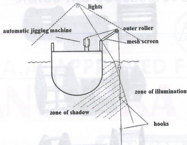
Fig. 5 General arrangement for jigging operation
