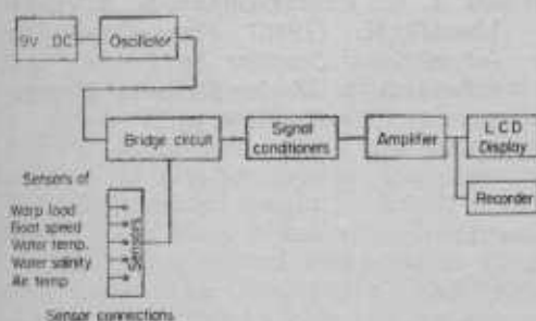
Fig. 3. Block diagram of fishing log
