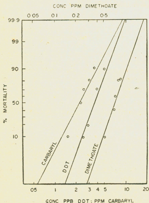
Fig. 1. Toxicity curves of the pesticides - Log-probit analysis
