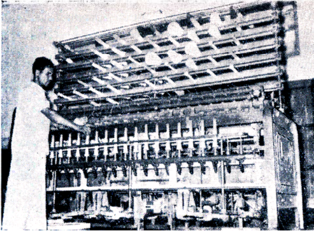
Twine twisting machine
