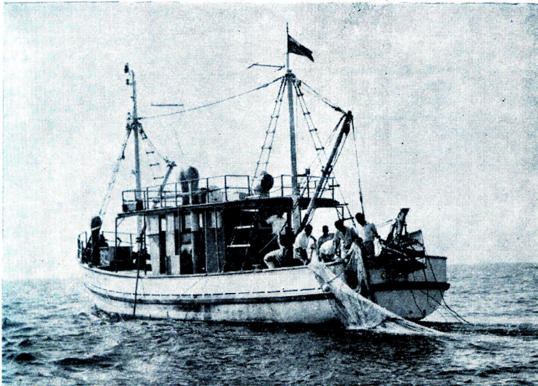
"Sindhukumari" — Cheaper version of CIFT prototype boat - 50' OAL - built in 1966. 30% cheaper than the conventional hull.
