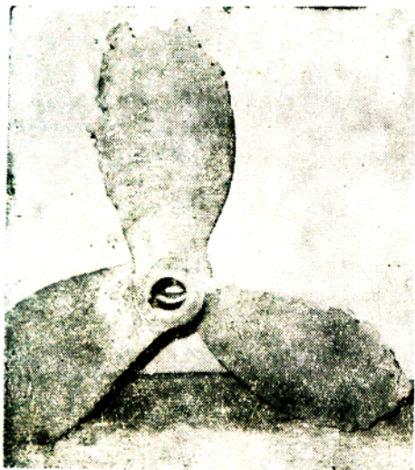
Marine Corrosion - Propeller
