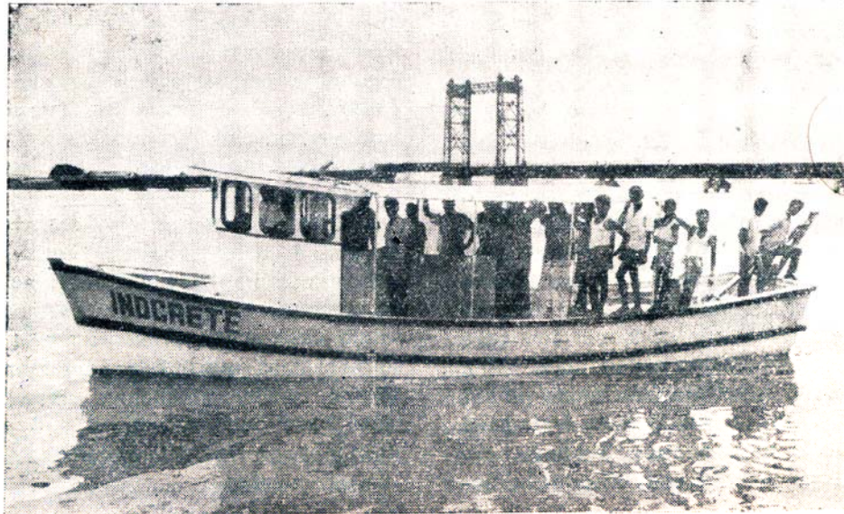
Ferrocement Boat - 'INDCRETE'
