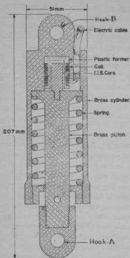
Fig. 1 UNDER WATER TENSION TRANSDUCER
