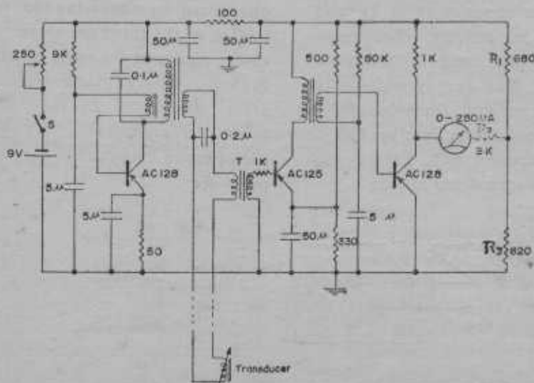
Fig. 2. Electronic circuit of the instrument.
