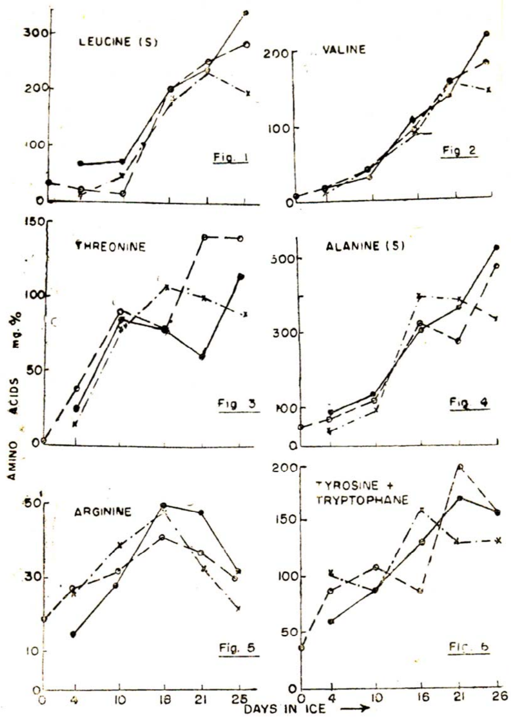
○ — — — ○ C = CONTROL ● — — — ● T 1 = FISH TREATED WITH 20 ppm. AUREOMYCIN, x, — — — x T 2 = FISH TREATED WITH 50 ppm AUREOMYCIN.
